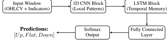
Figure 1: Architecture of the proposed hybrid CNN-LSTM model.
